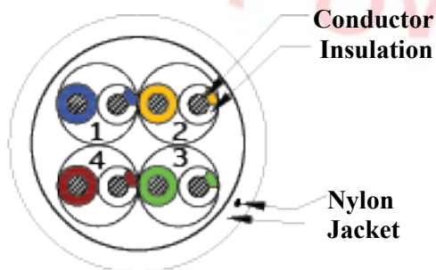
CROSS-SECTION
